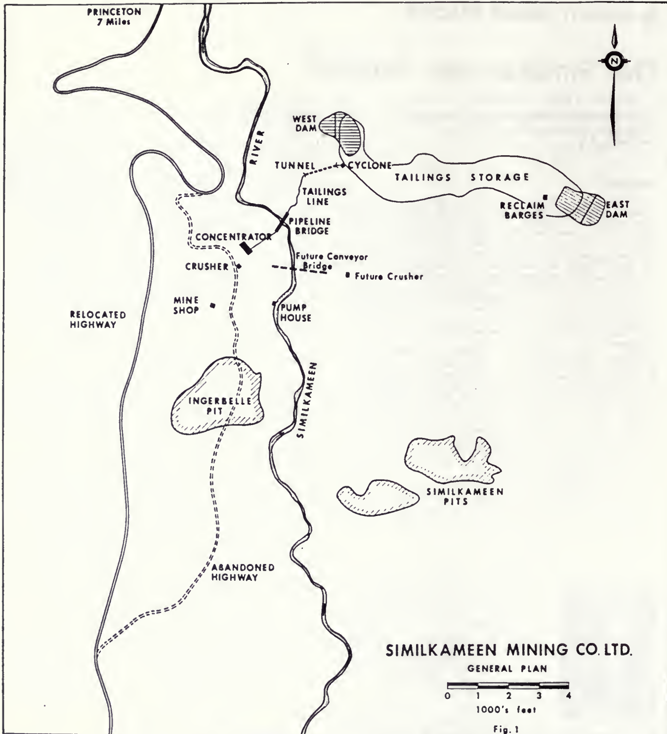
FIGURE 1 — General Plan — S.milkameen.
